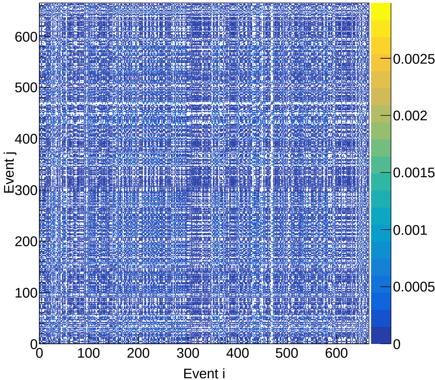
LH2 (total) Covariance | M: [4.2, 4.5) xF: [0.45, 0.50)
