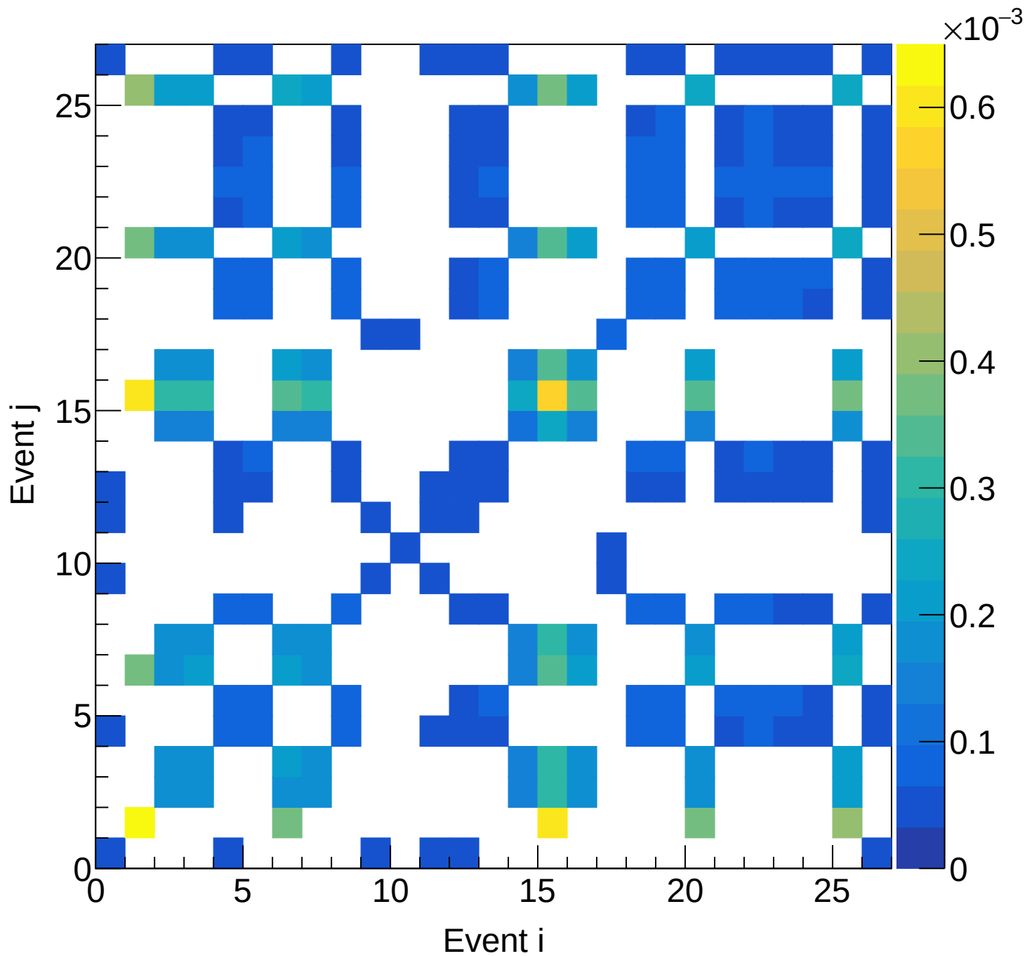
LH2 (total) Covariance | M: [6.9, 7.5) xF: [0.45, 0.50)
