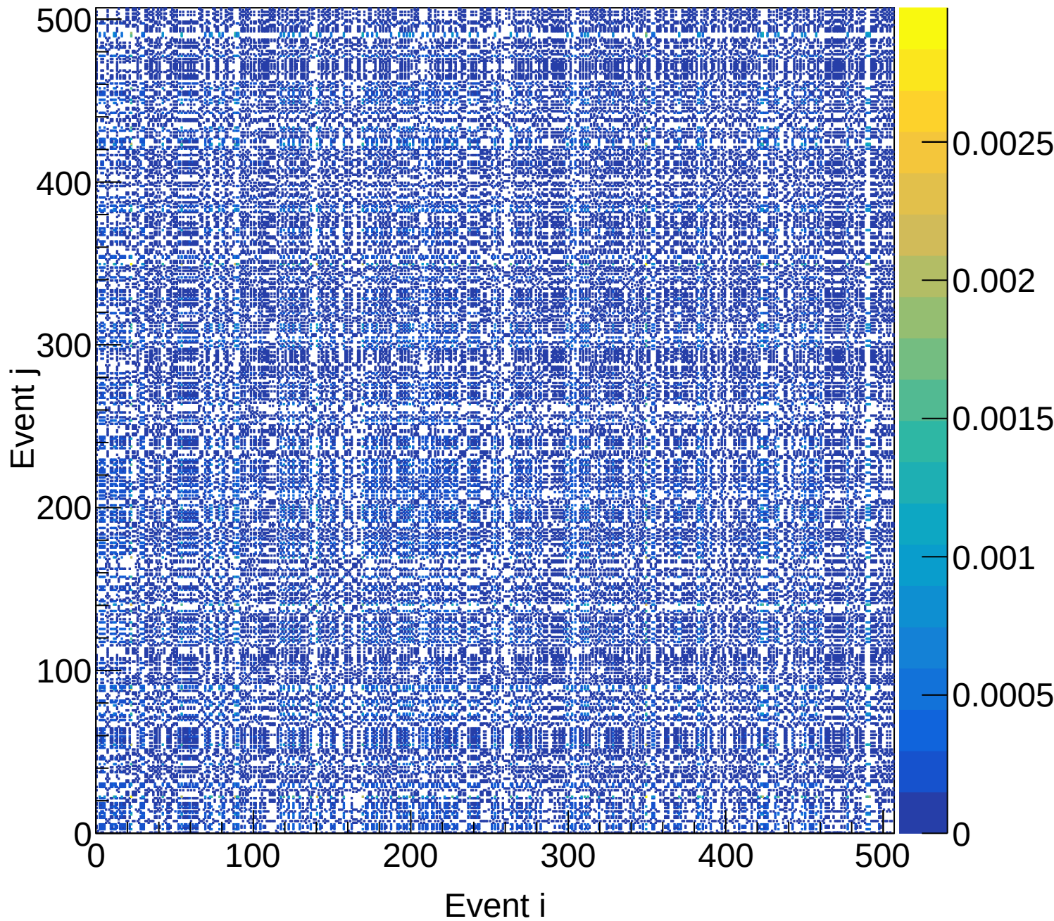
LH2 (total) Covariance | M: [4.5, 4.8) xF: [0.45, 0.50)
