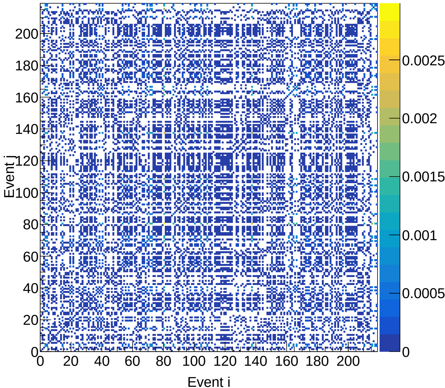
LH2 (total) Covariance | M: [5.1, 5.4) xF: [0.45, 0.50)
