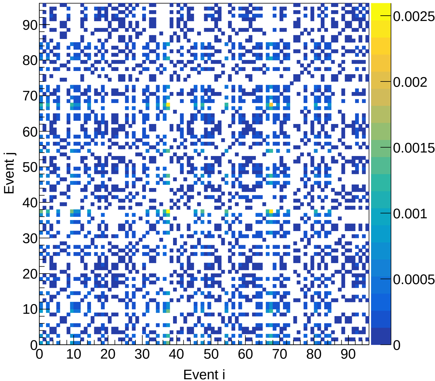
LH2 (total) Covariance | M: [5.7, 6.0) xF: [0.45, 0.50)
