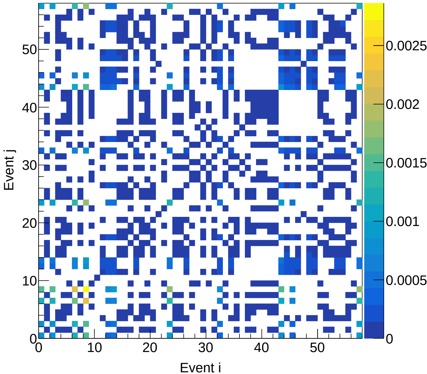
LH2 (total) Covariance | M: [6.0, 6.3) xF: [0.45, 0.50)
