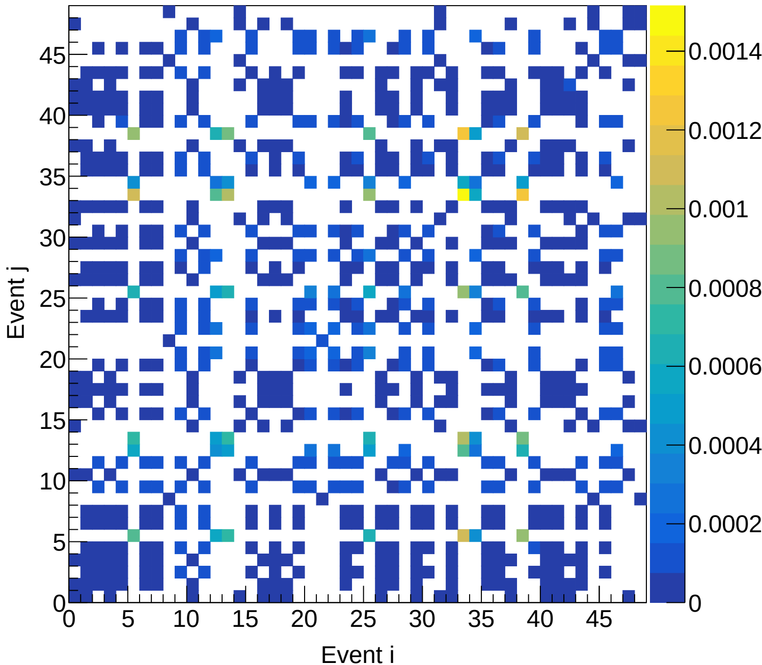
LH2 (total) Covariance | M: [6.3, 6.6] xF: [0.45, 0.50)
