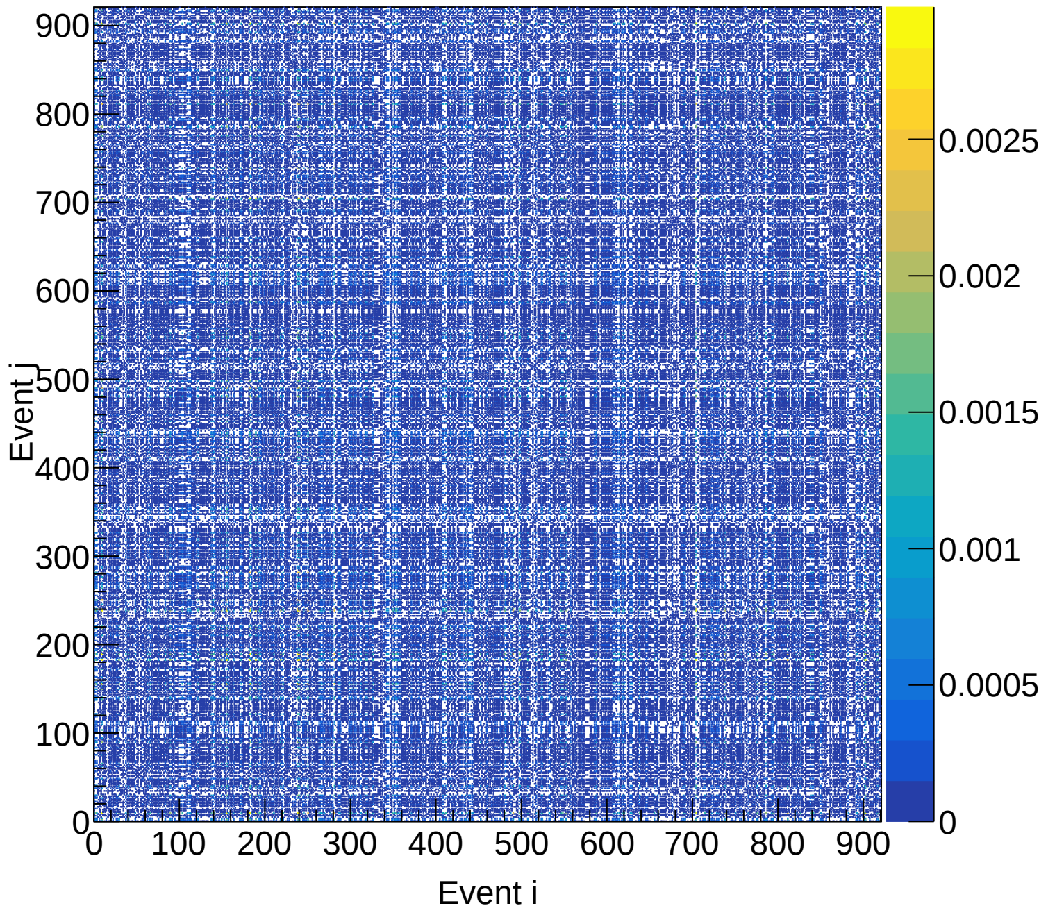
LH2 (total) Covariance | M: [3.9, 4.2) xF: [0.50, 0.55)
