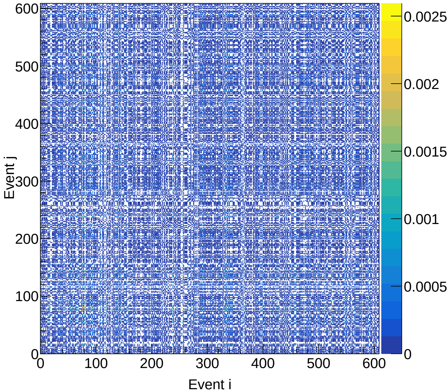
LH2 (total) Covariance | M: [4.2, 4.5) xF: [0.50, 0.55)
