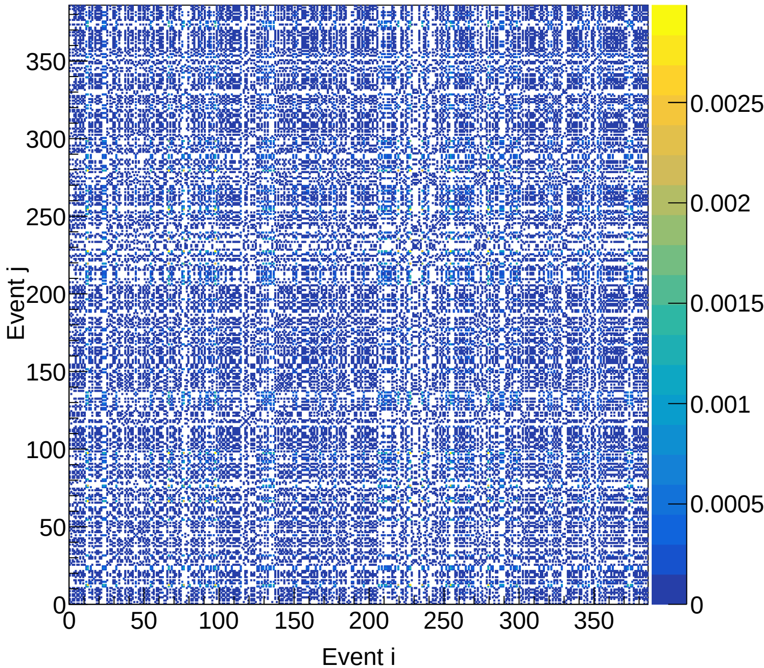
LH2 (total) Covariance | M: [4.5, 4.8) xF: [0.50, 0.55)
