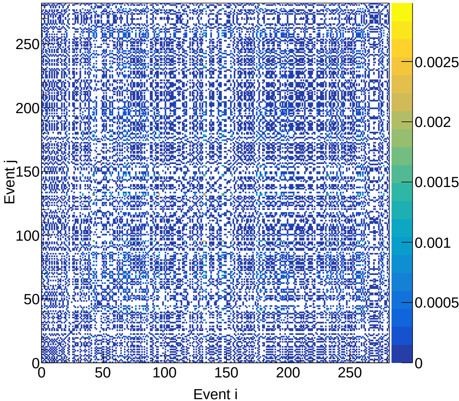
LH2 (total) Covariance | M: [4.8, 5.1) xF: [0.50, 0.55)
