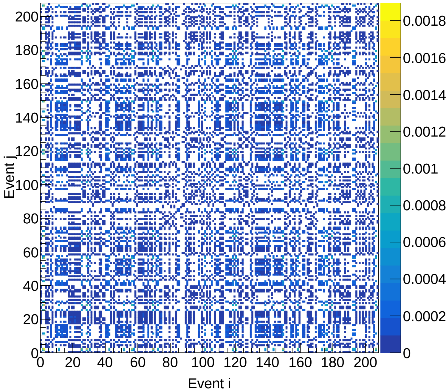
LH2 (total) Covariance | M: [5.1, 5.4) xF: [0.50, 0.55)
