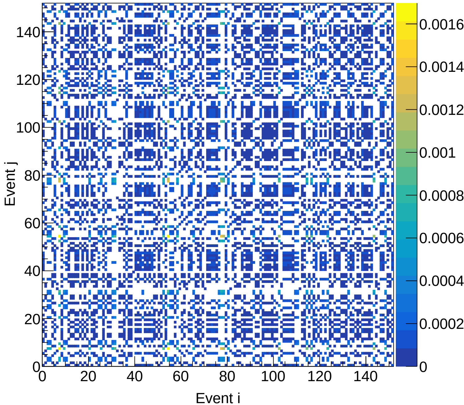
LH2 (total) Covariance | M: [5.4, 5.7) xF: [0.50, 0.55)
