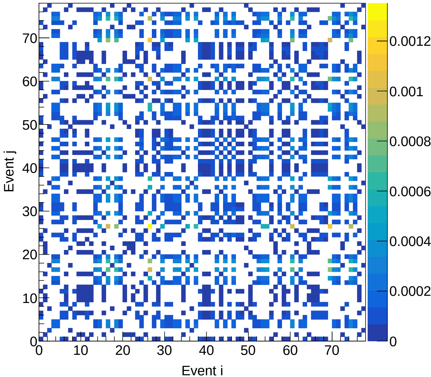
LH2 (total) Covariance | M: [5.7, 6.0) xF: [0.50, 0.55)
