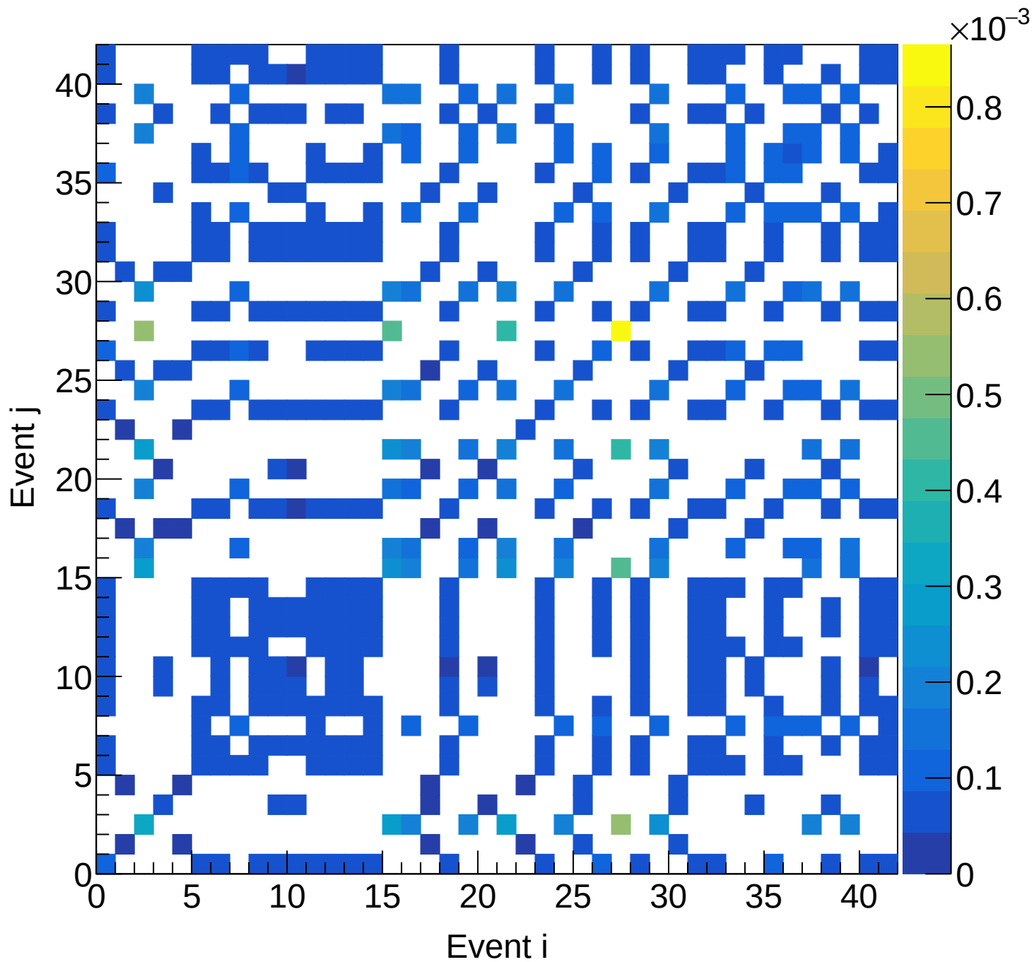
LH2 (total) Covariance | M: [6.0, 6.3) xF: [0.50, 0.55)
