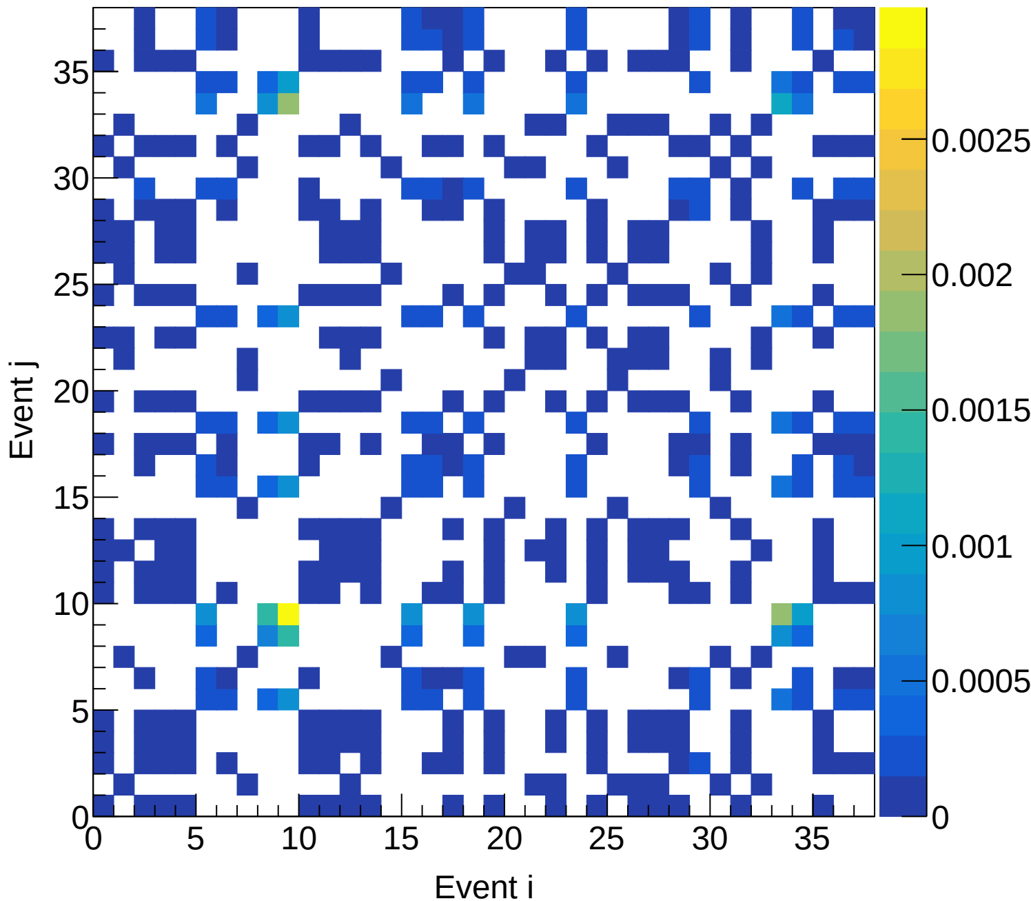
LH2 (total) Covariance | M: [6.3, 6.6) xF: [0.50, 0.55)
