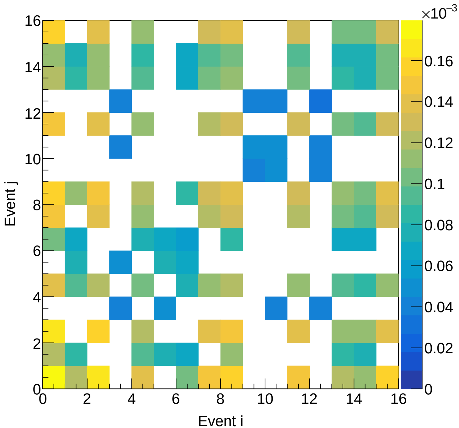
LH2 (total) Covariance | M: [6.6, 6.9] xF: [0.50, 0.55]
