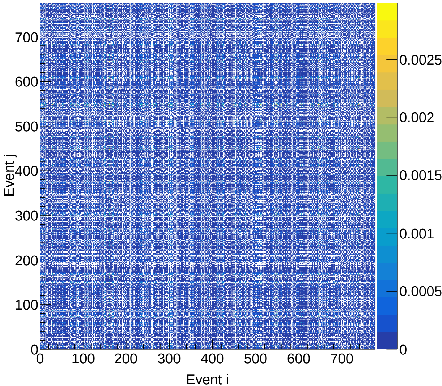
LH2 (total) Covariance | M: [3.9, 4.2) xF: [0.55, 0.60)
