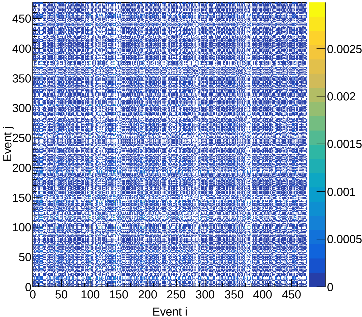
LH2 (total) Covariance | M: [4.2, 4.5) xF: [0.55, 0.60)
