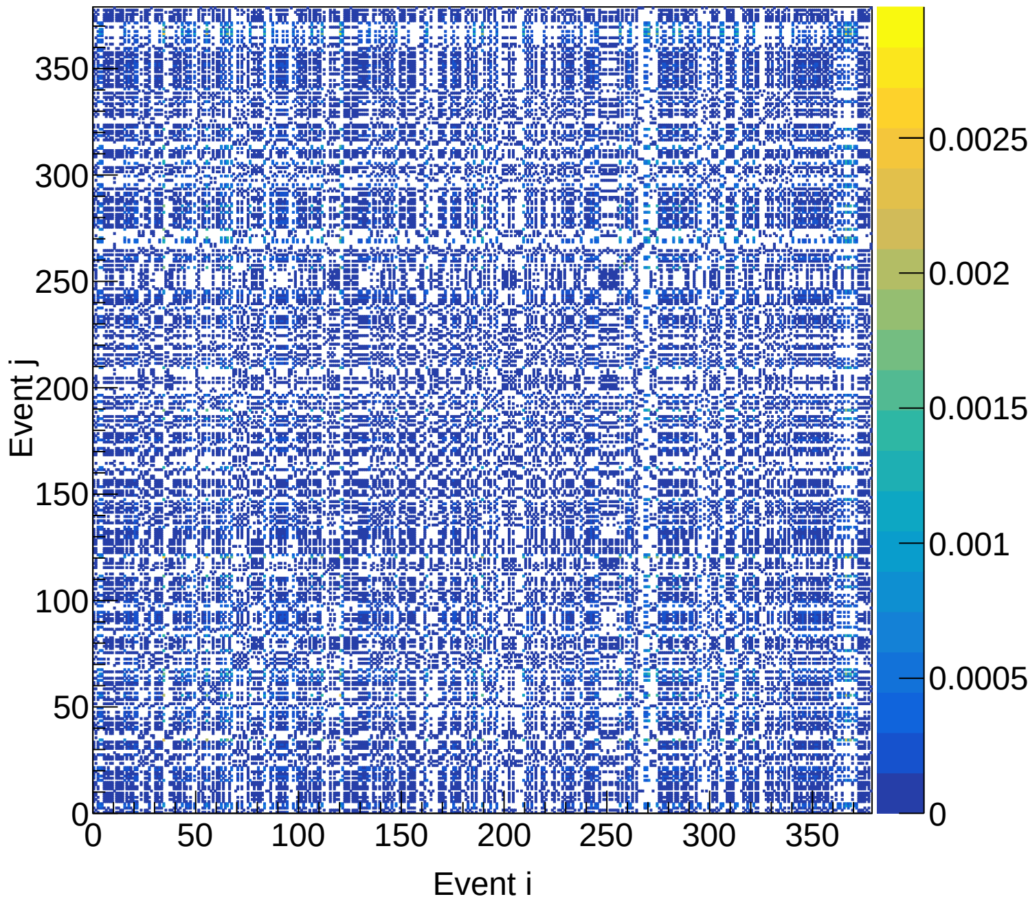
LH2 (total) Covariance | M: [4.5, 4.8) xF: [0.55, 0.60)
