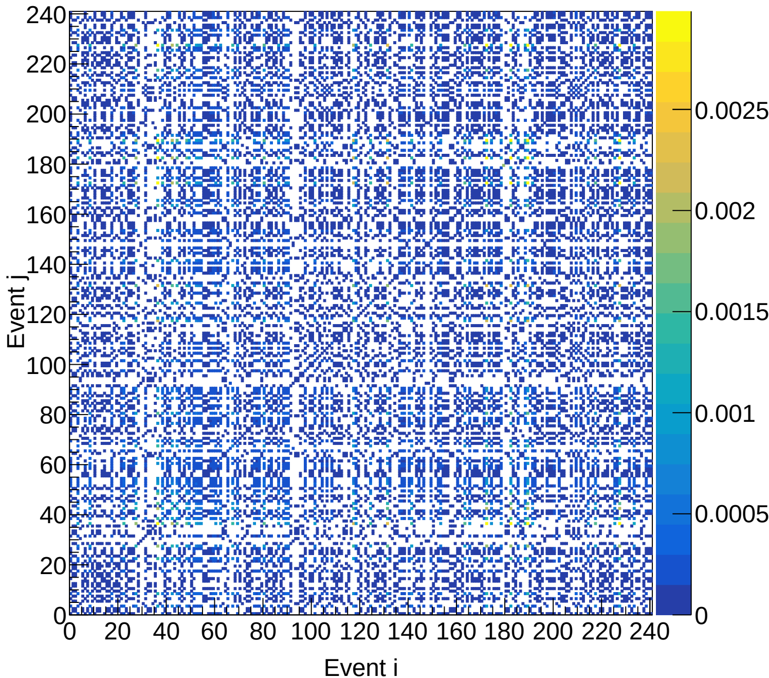
LH2 (total) Covariance | M: [4.8, 5.1) xF: [0.55, 0.60)
