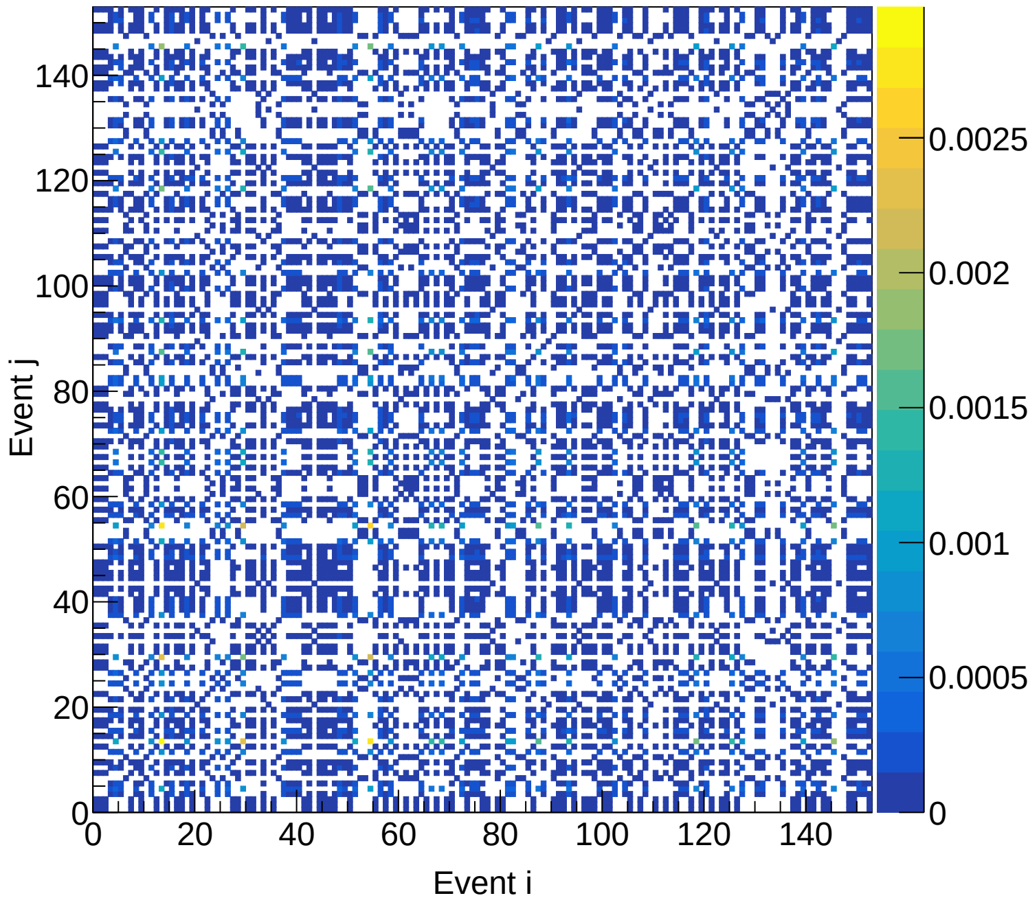
LH2 (total) Covariance | M: [5.1, 5.4) xF: [0.55, 0.60)
