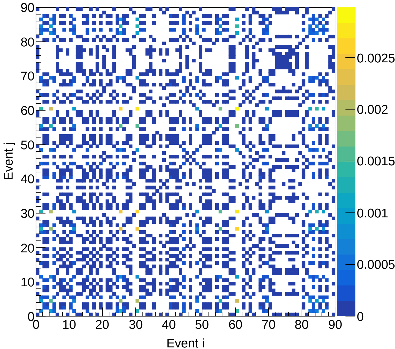
LH2 (total) Covariance | M: [5.4, 5.7) xF: [0.55, 0.60)
