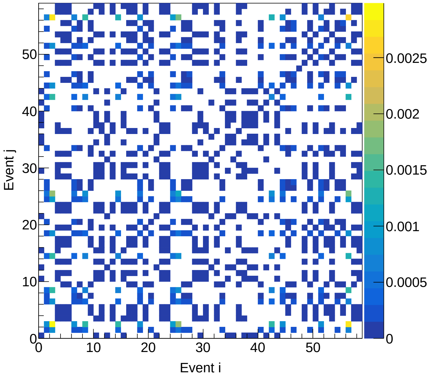
LH2 (total) Covariance | M: [5.7, 6.0] xF: [0.55, 0.60]
