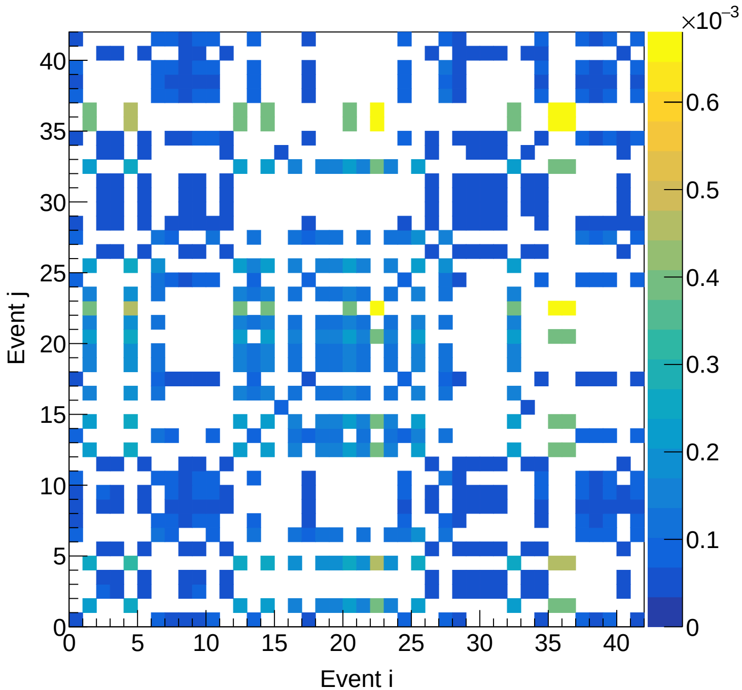
LH2 (total) Covariance | M: [6.0, 6.3) xF: [0.55, 0.60)
