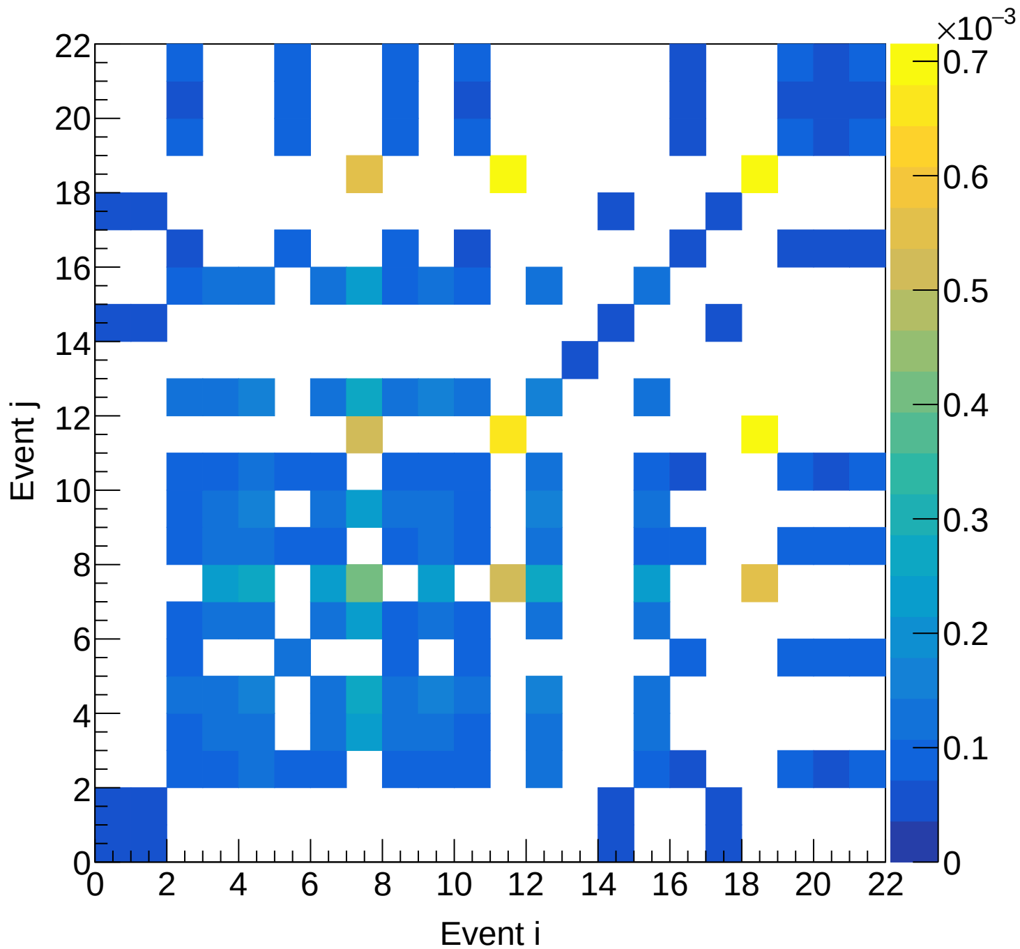
LH2 (total) Covariance | M: [6.3, 6.6) xF: [0.55, 0.60)
