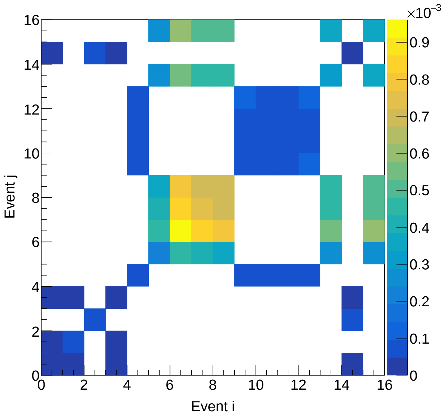
LH2 (total) Covariance | M: [6.6, 6.9] xF: [0.55, 0.60)
