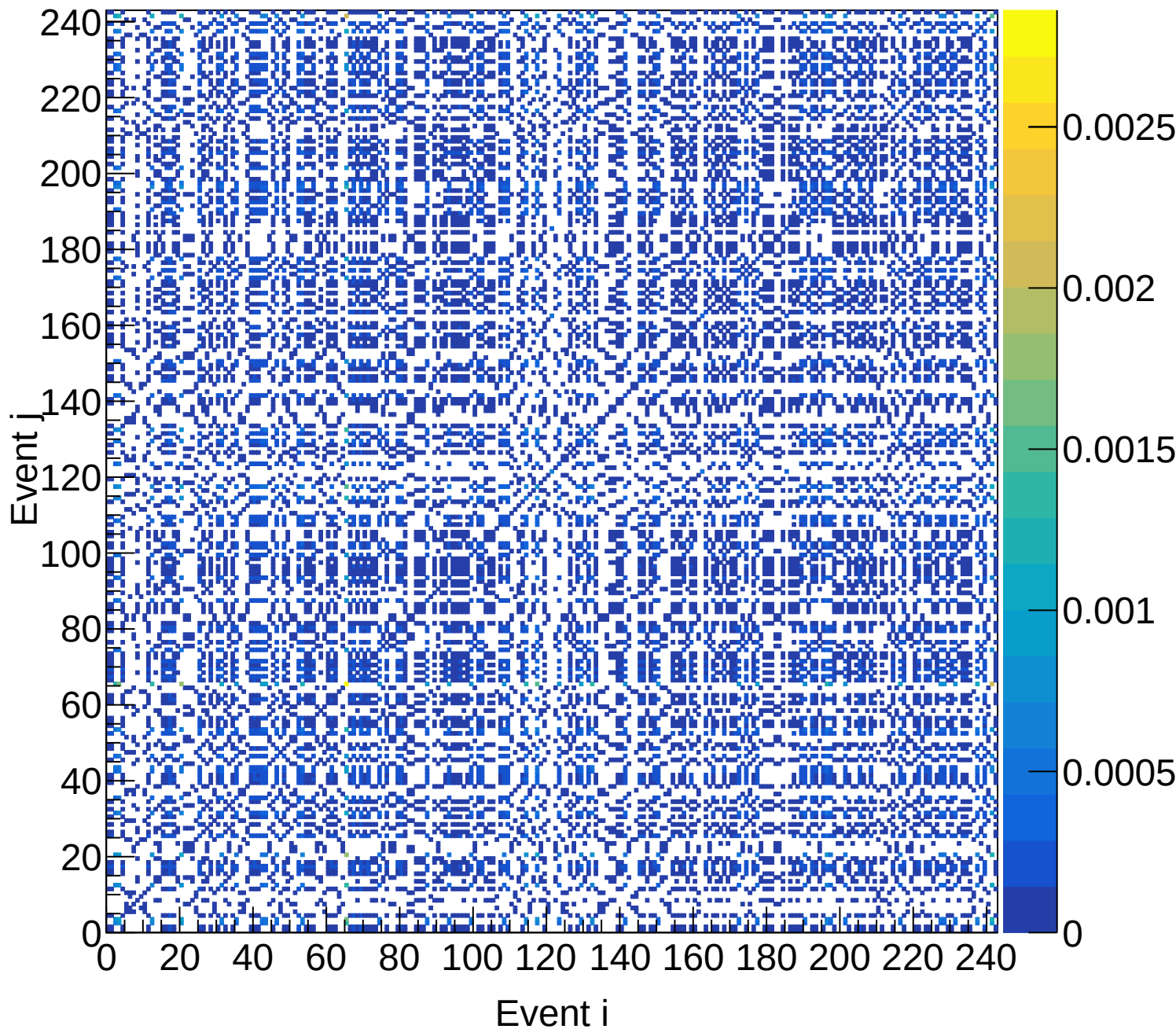
LH2 (total) Covariance | M: [4.5, 4.8) xF: [0.60, 0.65)
