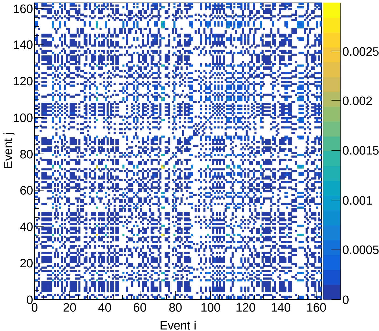
LH2 (total) Covariance | M: [4.8, 5.1) xF: [0.60, 0.65)
