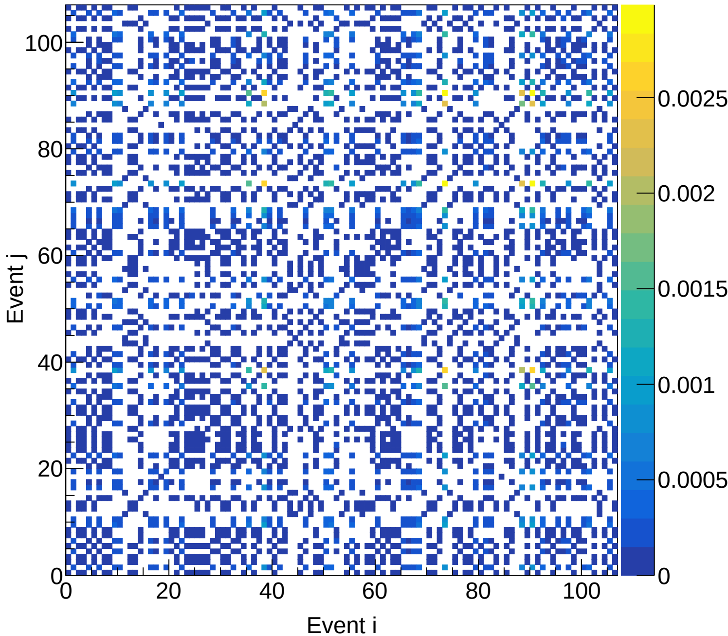
LH2 (total) Covariance | M: [5.1, 5.4) xF: [0.60, 0.65)
