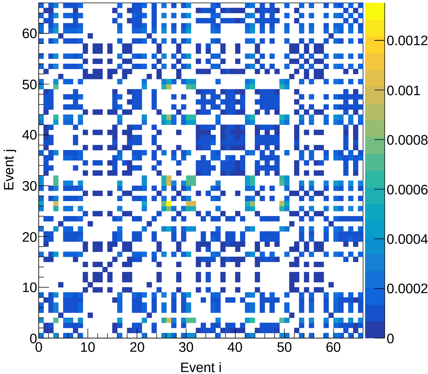
LH2 (total) Covariance | M: [5.4, 5.7) xF: [0.60, 0.65)
