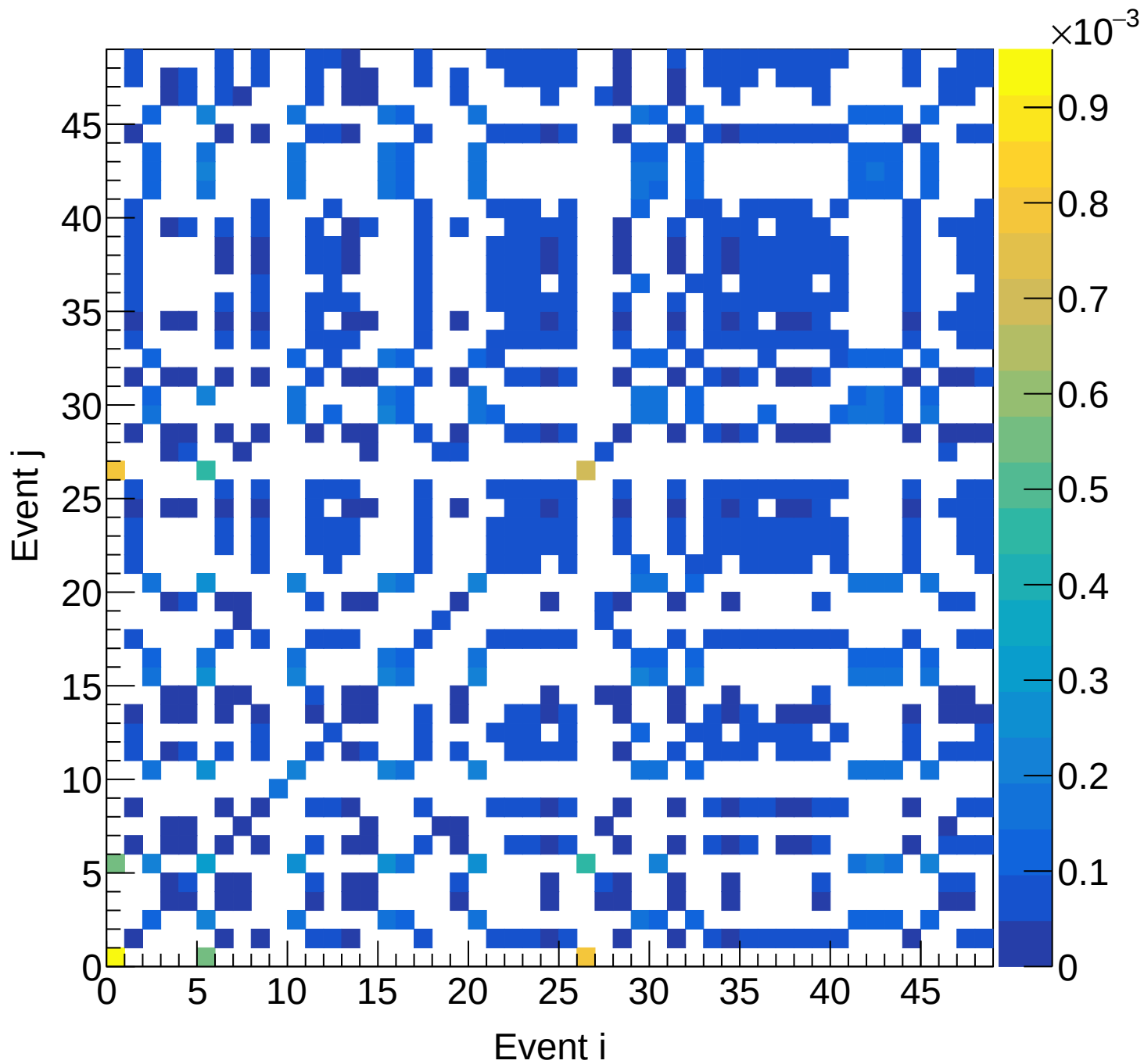
LH2 (total) Covariance | M: [5.7, 6.0] xF: [0.60, 0.65]
