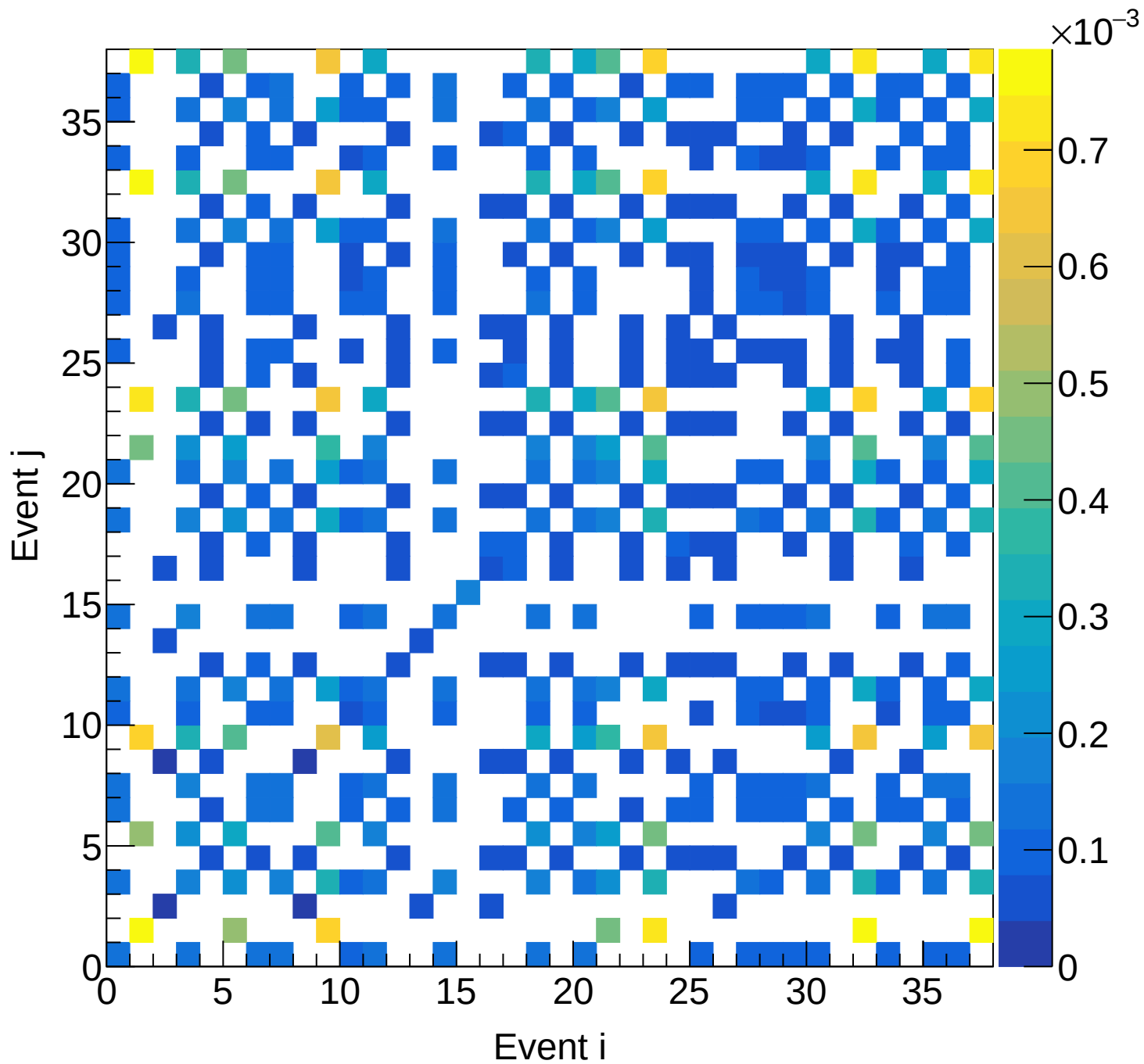
LH2 (total) Covariance | M: [6.0, 6.3) xF: [0.60, 0.65)
