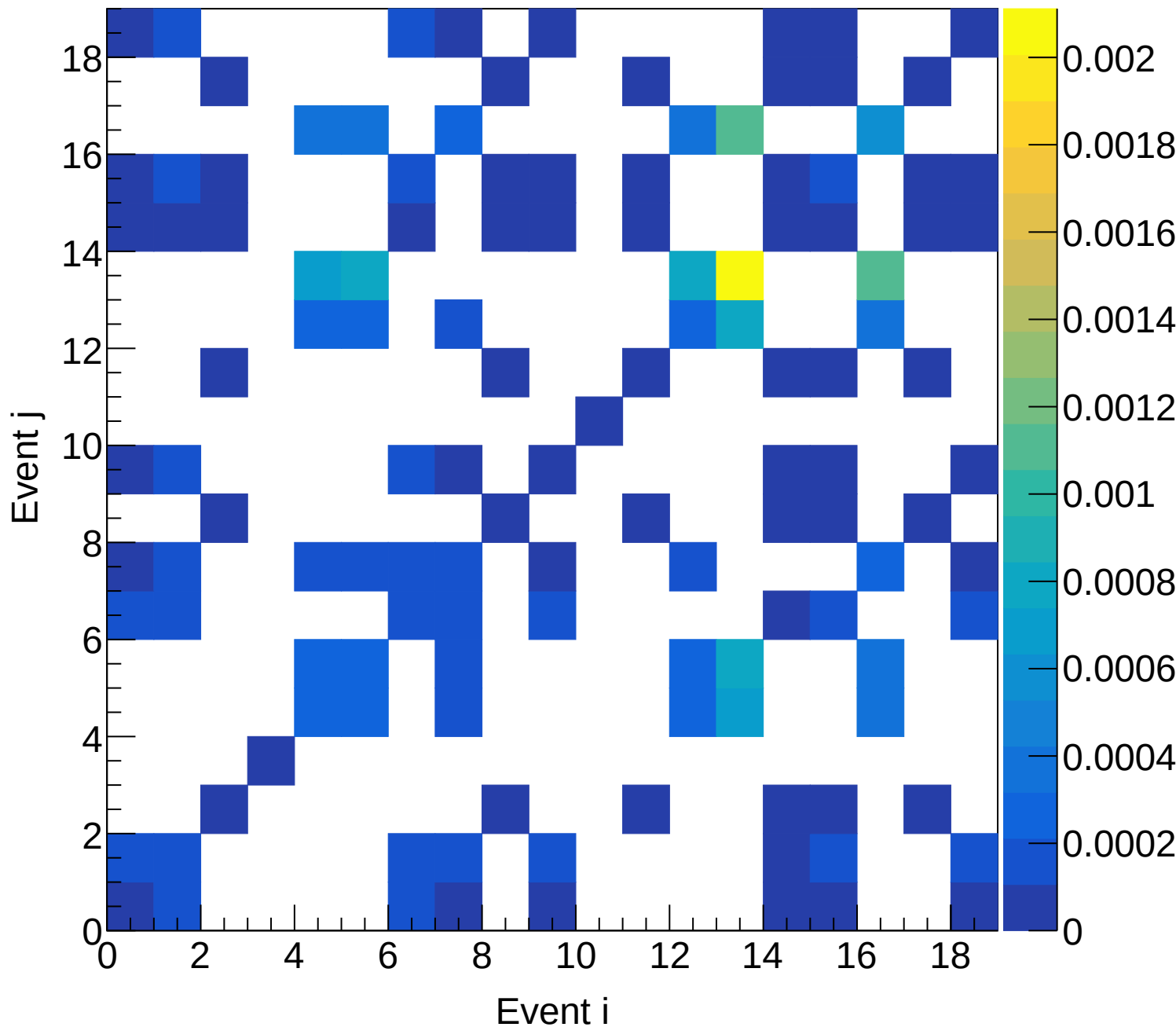
LH2 (total) Covariance | M: [6.3, 6.6) xF: [0.60, 0.65)
