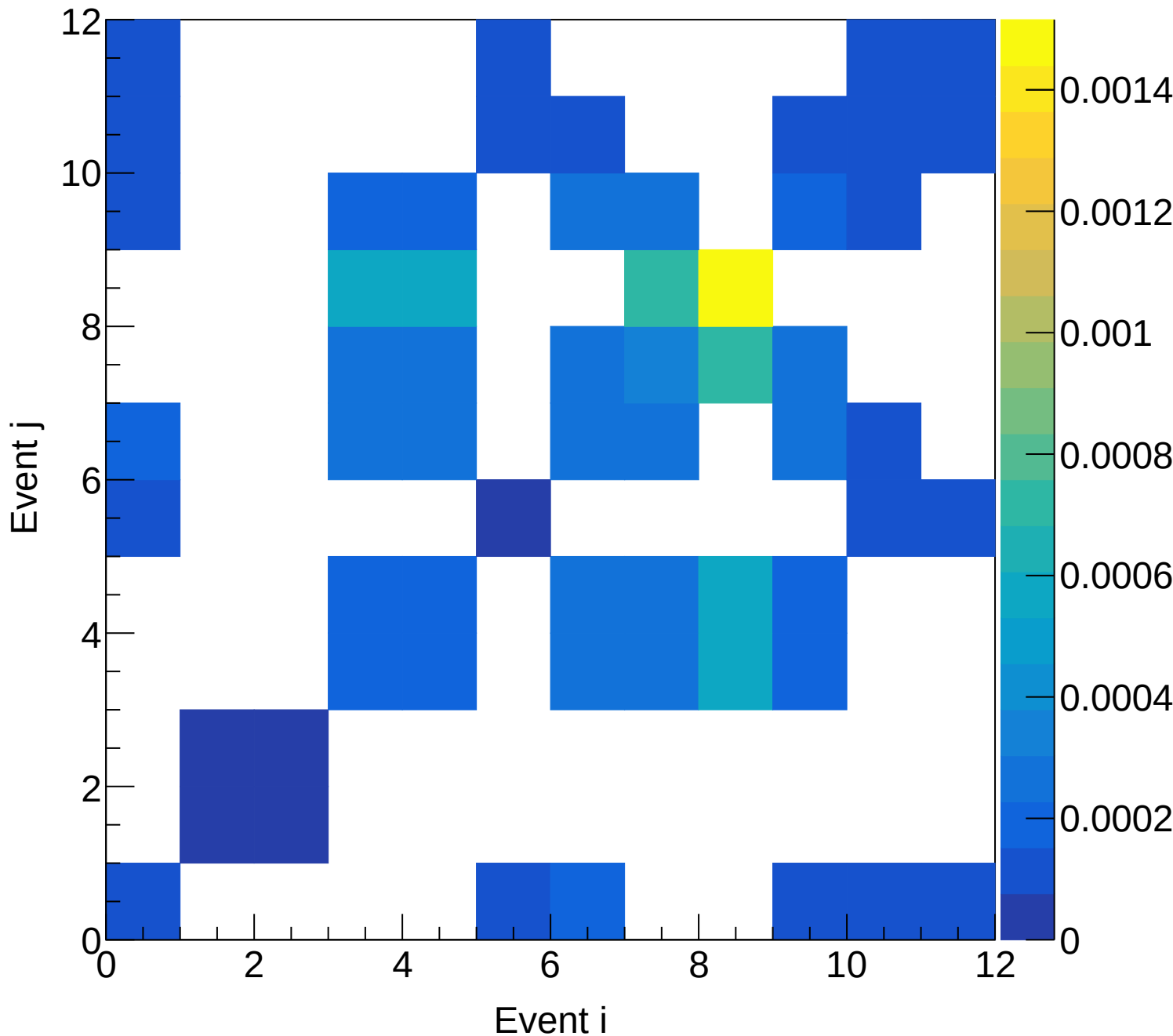
LH2 (total) Covariance | M: [6.6, 6.9) xF: [0.60, 0.65)
