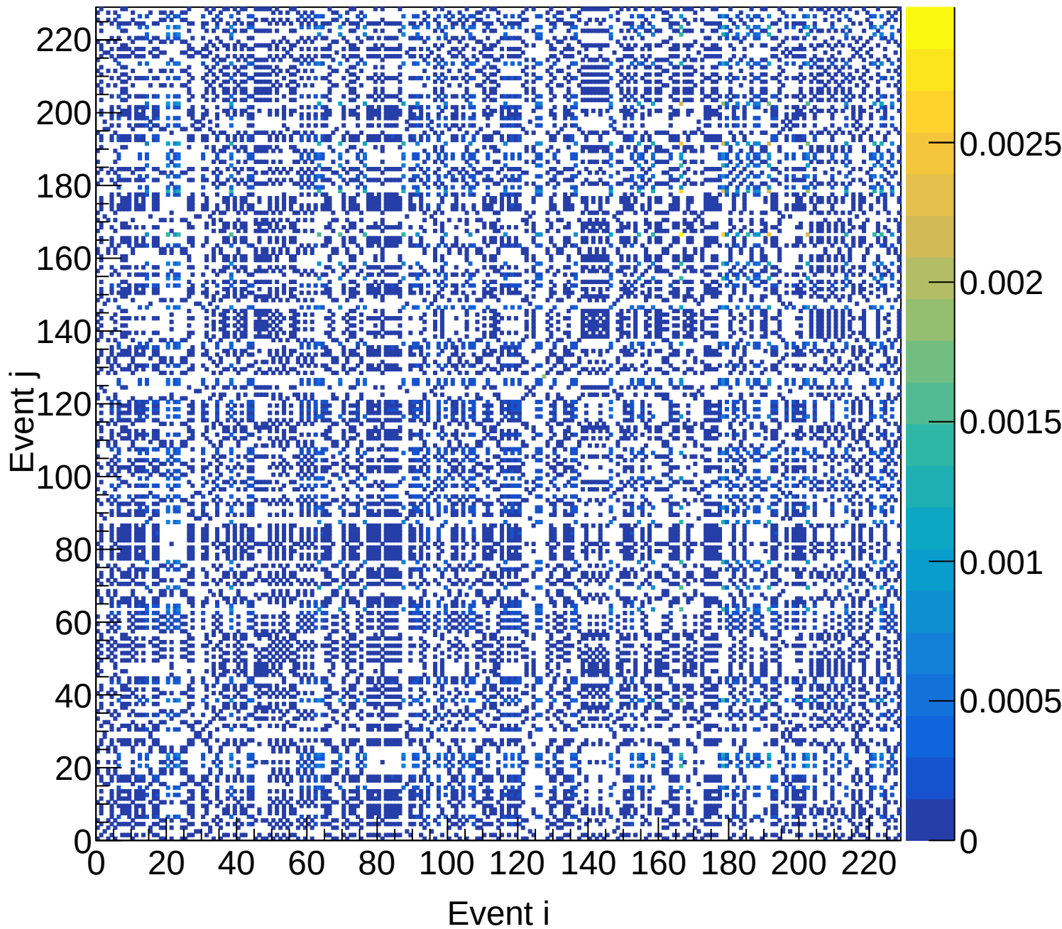
LH2 (total) Covariance | M: [4.2, 4.5) xF: [0.65, 0.70)
