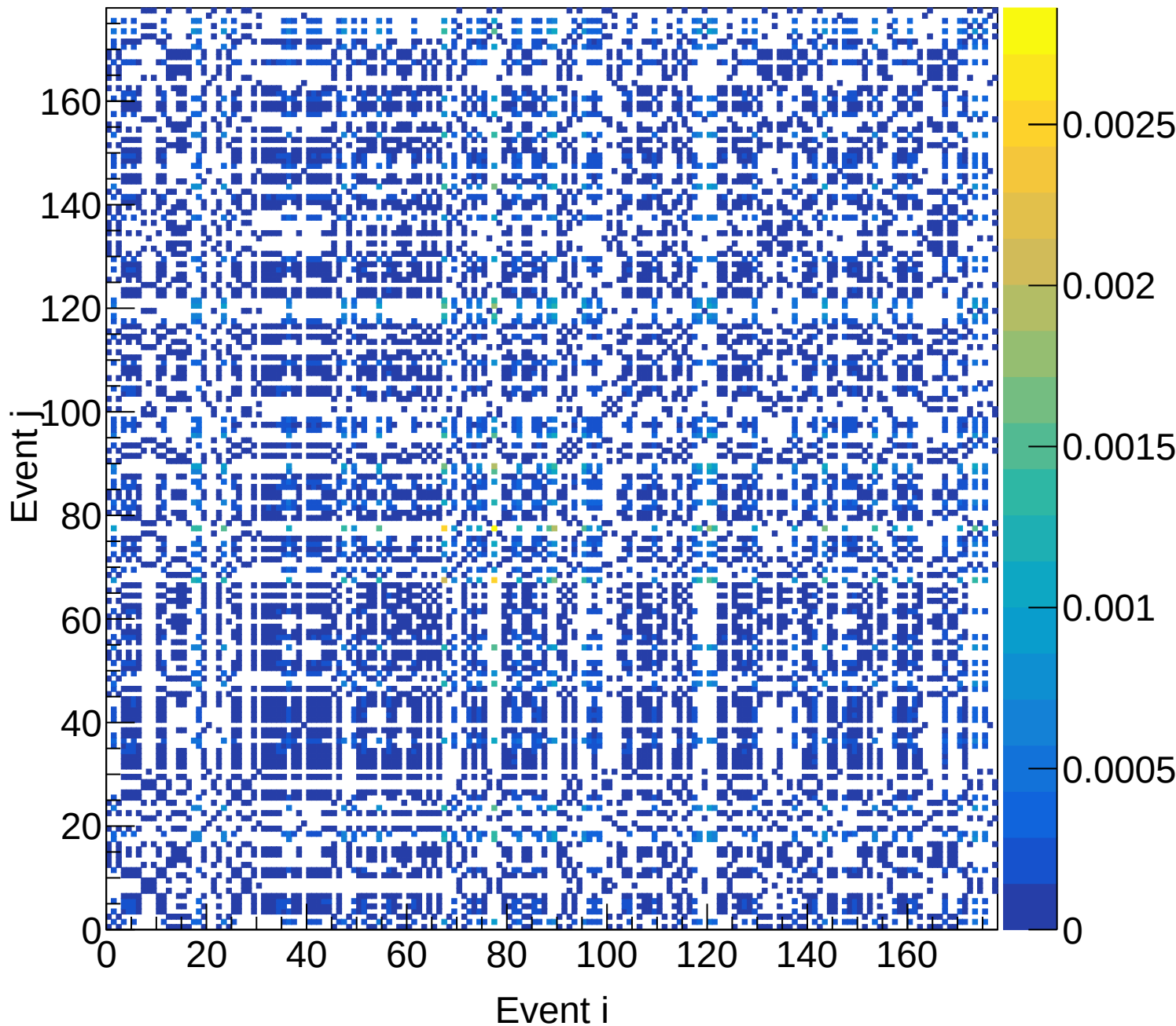
LH2 (total) Covariance | M: [4.5, 4.8) xF: [0.65, 0.70)
