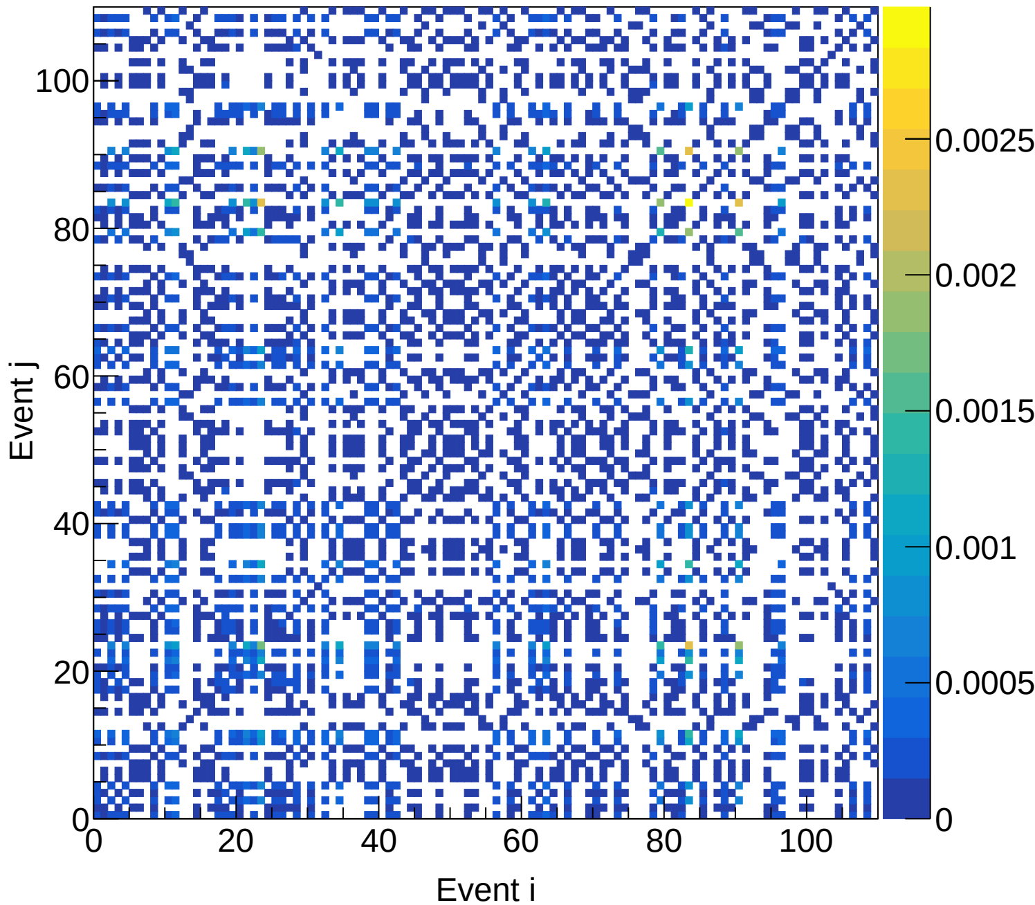
LH2 (total) Covariance | M: [4.8, 5.1) xF: [0.65, 0.70)
