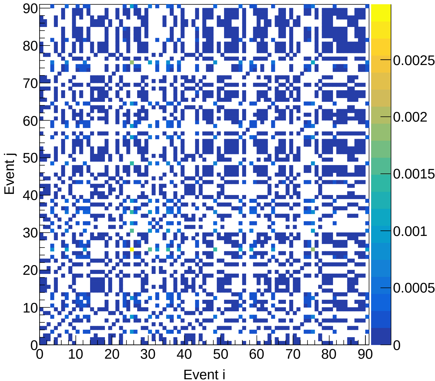
LH2 (total) Covariance | M: [5.1, 5.4) xF: [0.65, 0.70)
