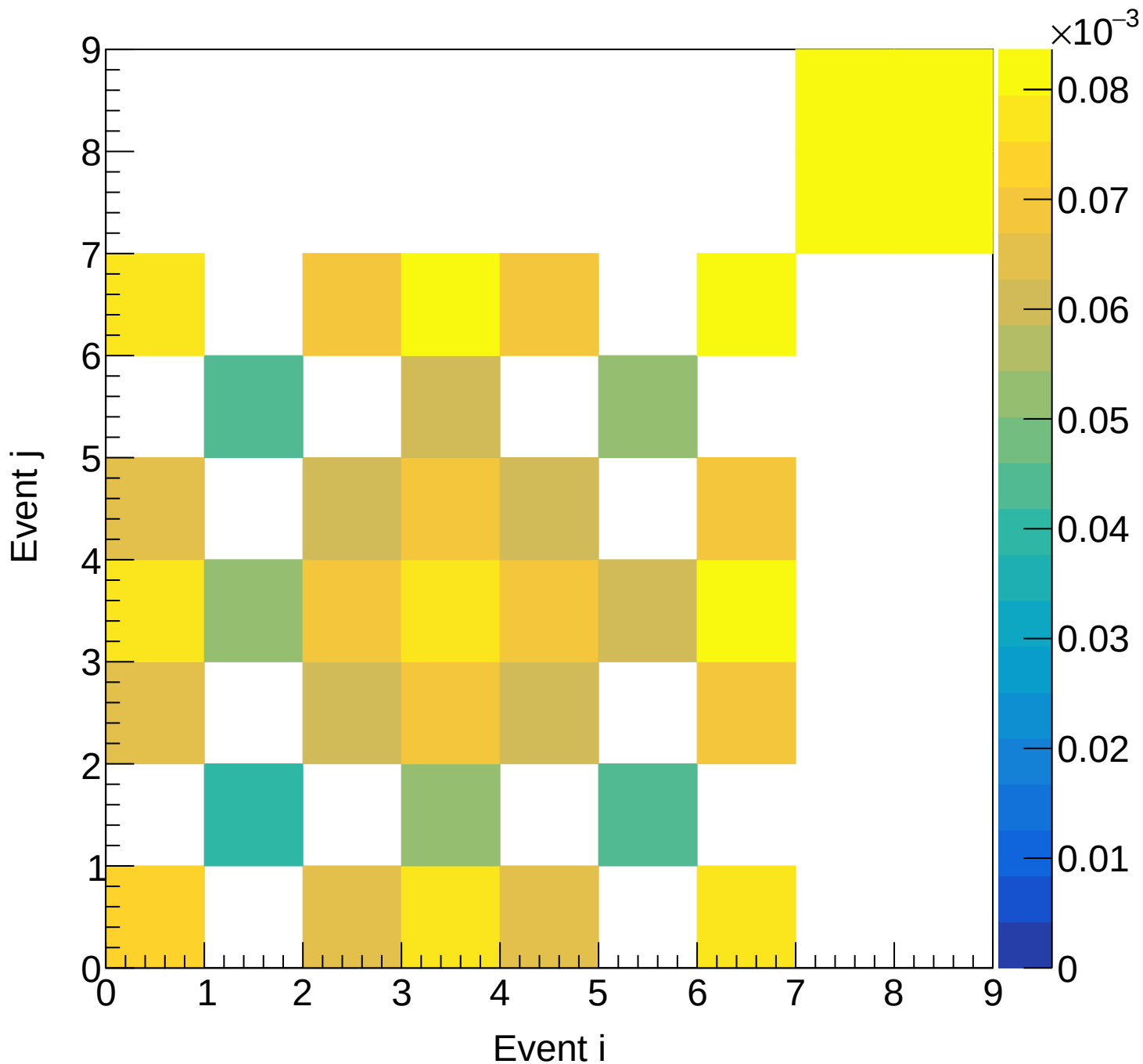
LH2 (total) Covariance | M: [6.3, 6.6) xF: [0.65, 0.70)
