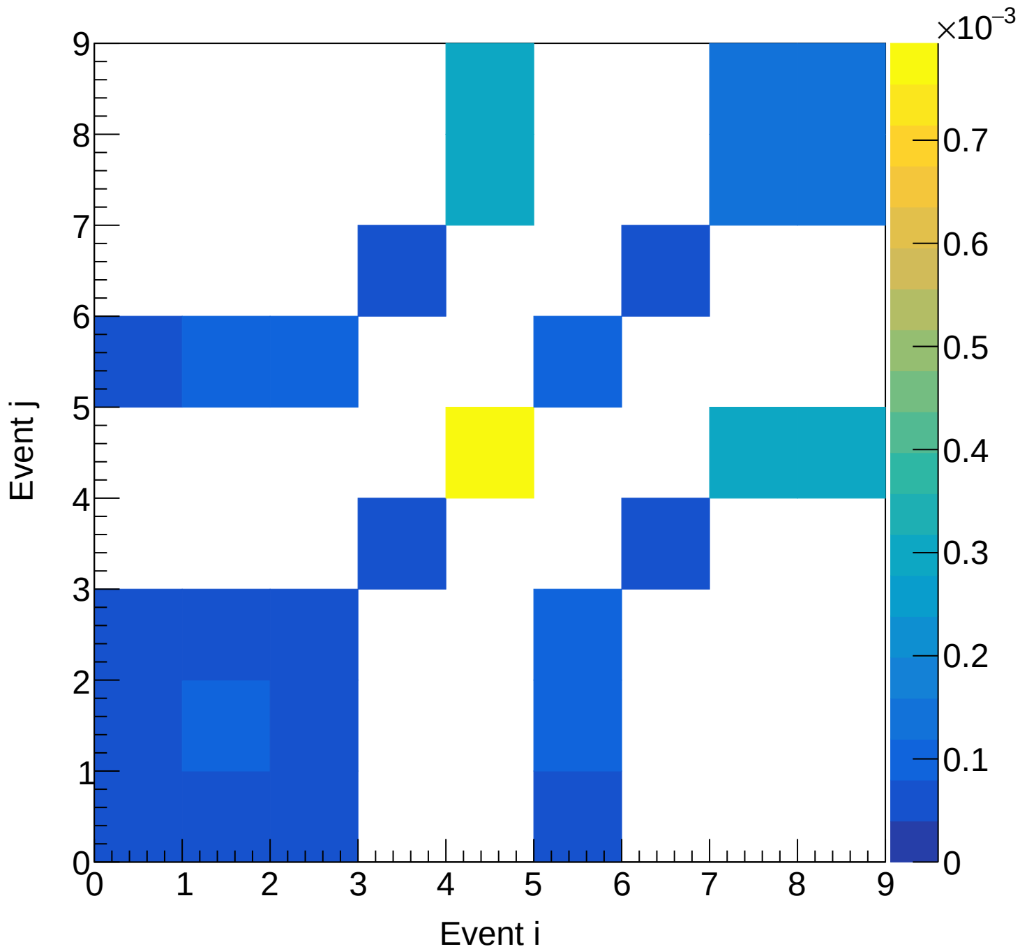
LH2 (total) Covariance | M: [6.6, 6.9] xF: [0.65, 0.70)
