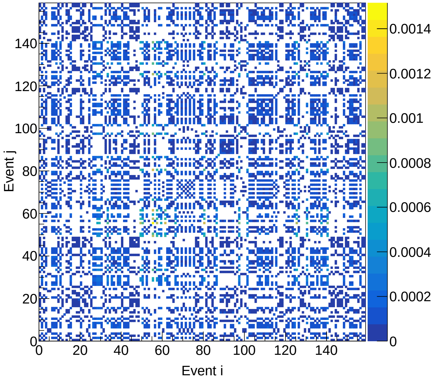
LH2 (total) Covariance | M: [4.2, 4.5] xF: [0.70, 0.75]
