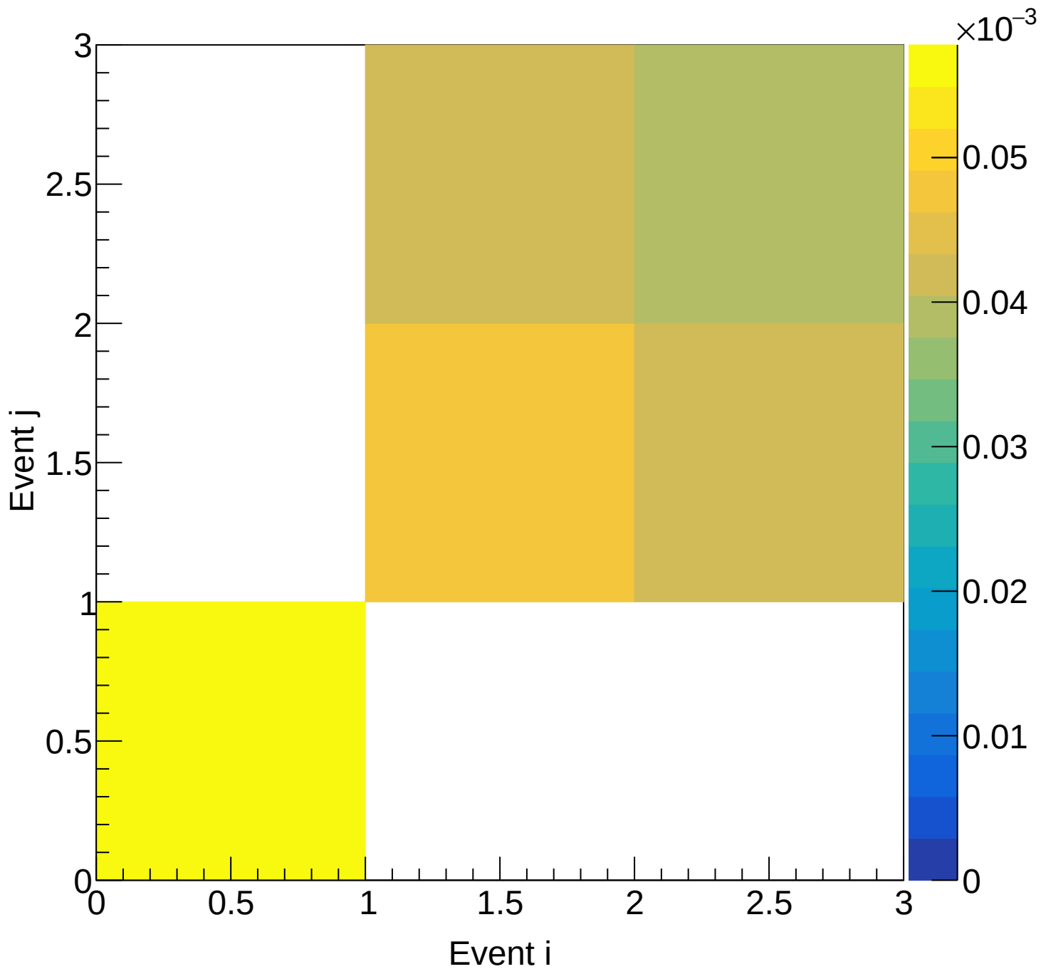
LH2 (total) Covariance | M: [6.9, 7.5) xF: [0.70, 0.75)
