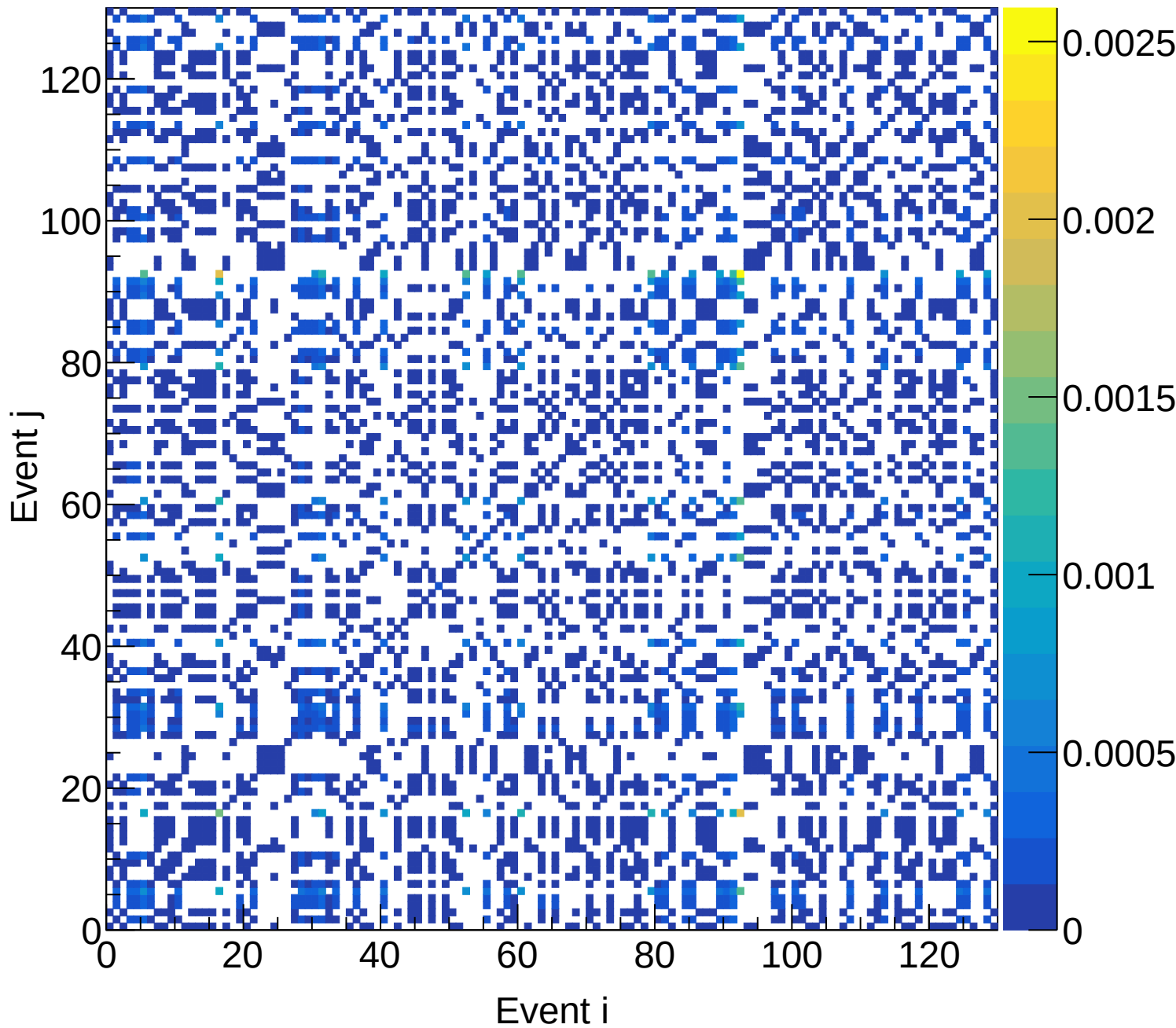
LH2 (total) Covariance | M: [4.5, 4.8) xF: [0.70, 0.75)
