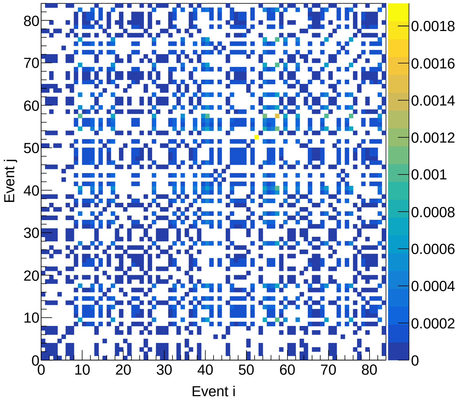
LH2 (total) Covariance | M: [4.8, 5.1) xF: [0.70, 0.75)
