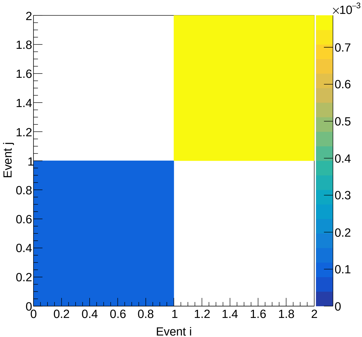
LH2 (total) Covariance | M: [4.2, 4.5) xF: [0.05, 0.10)
