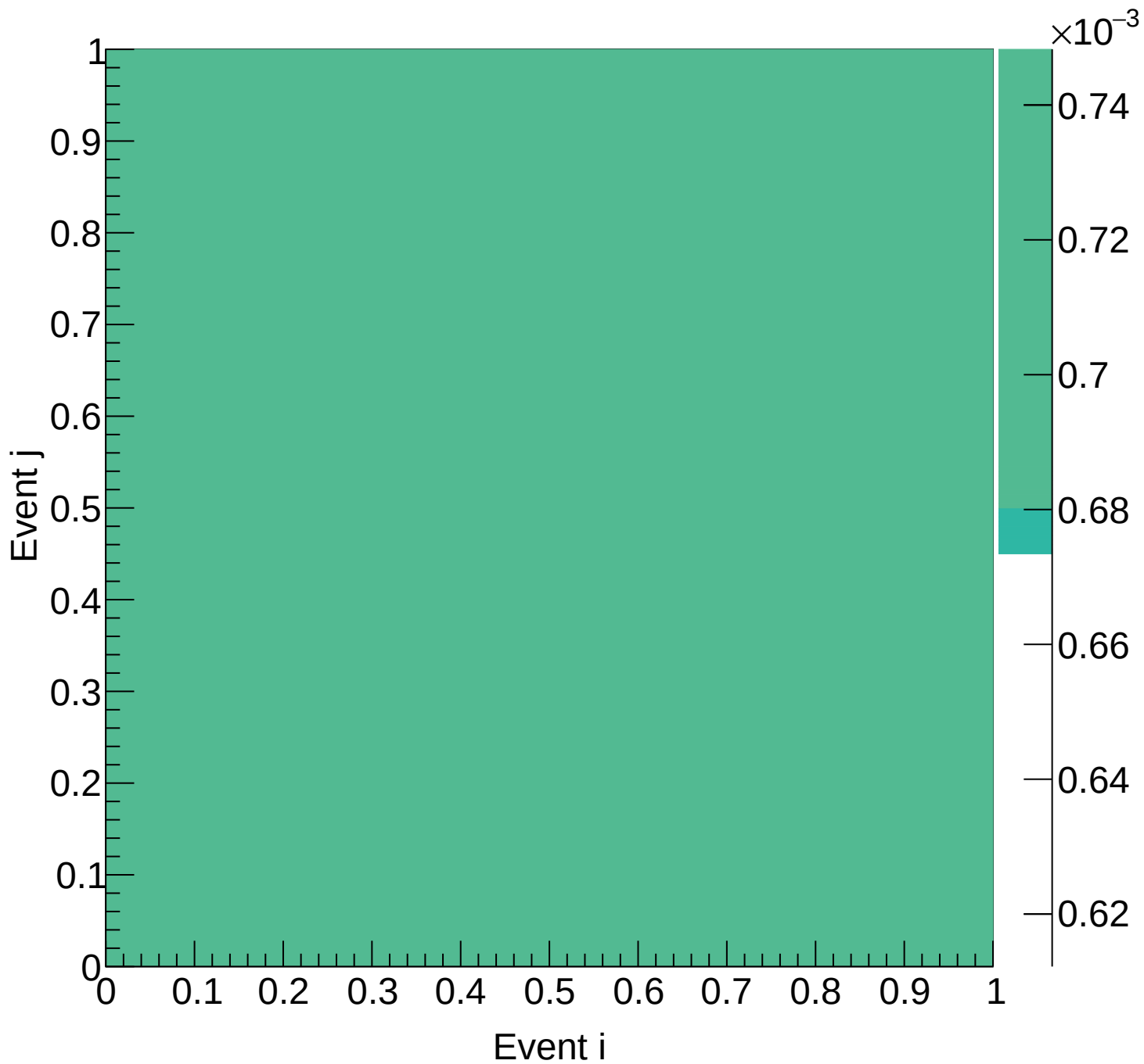
LH2 (total) Covariance | M: [4.2, 4.5) xF: [0.00, 0.05)
