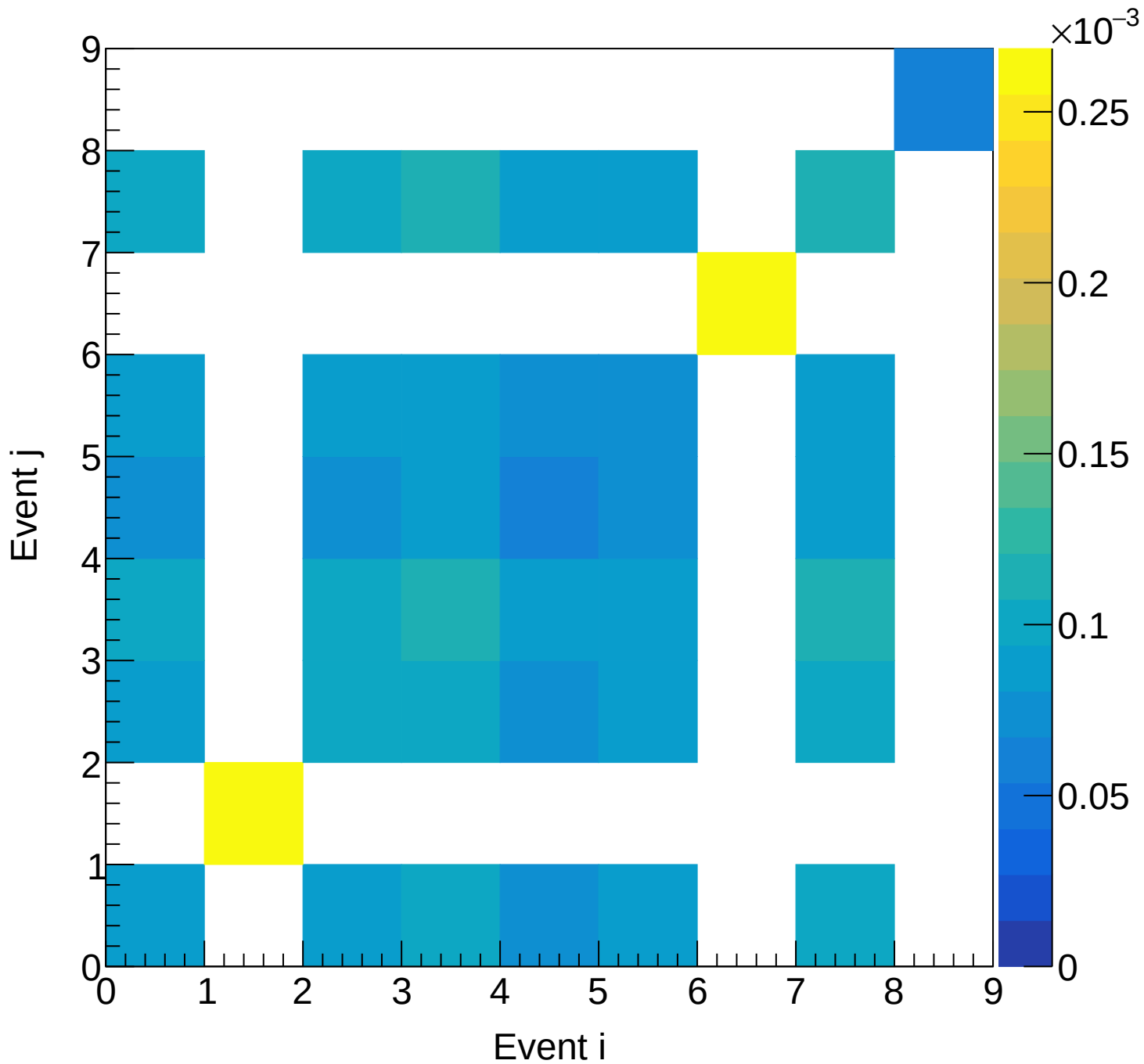
LH2 (total) Covariance | M: [6.9, 7.5] xF: [0.00, 0.05)
