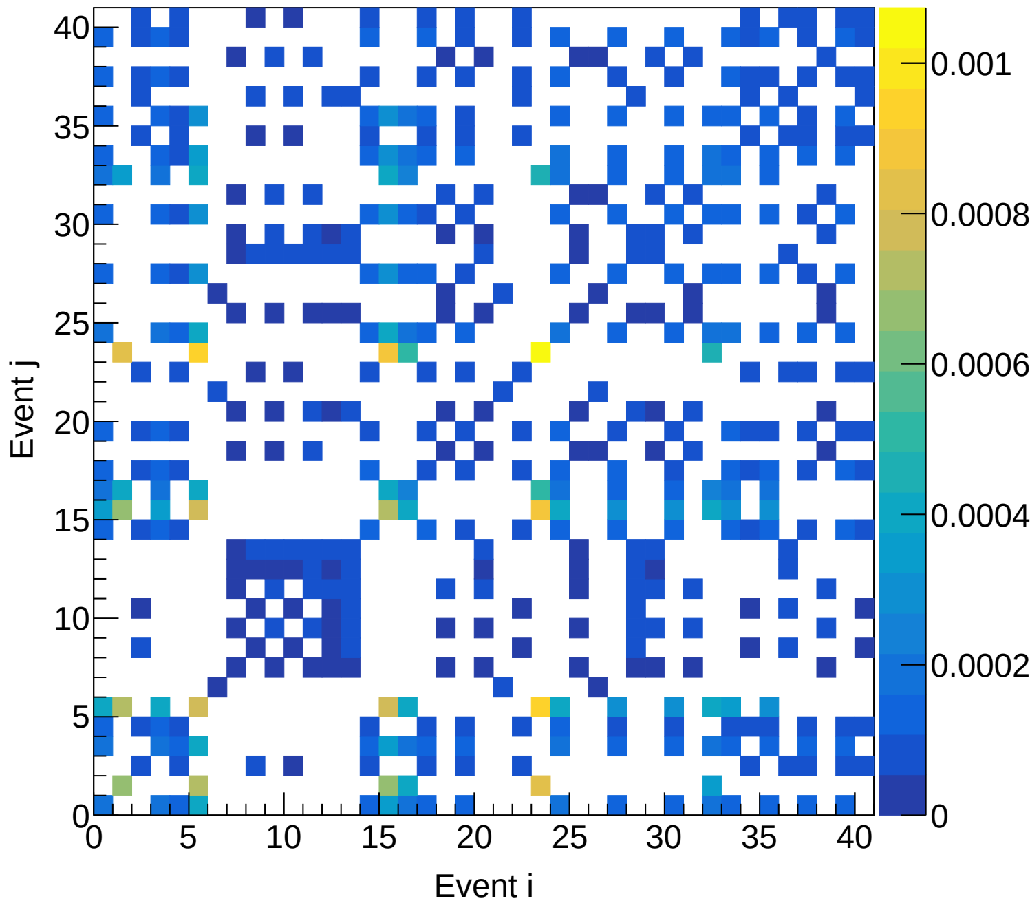
LH2 (total) Covariance | M: [4.8, 5.1) xF: [0.00, 0.05)
