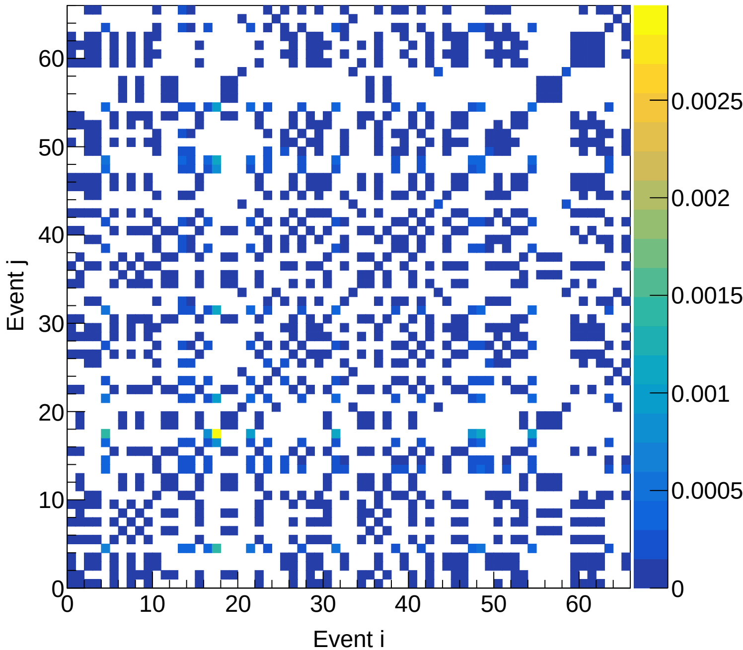
LH2 (total) Covariance | M: [5.4, 5.7) xF: [0.00, 0.05)
